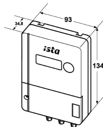
Abmessungen in mm: L = 134/B = 93/H = 35
