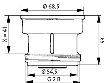
Dimensions prolongation*
