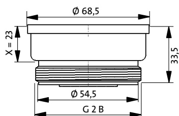
Dimensions prolongation*
